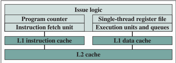
(a) Superscalar
