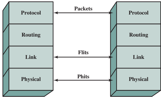
Figure 3.18 QPI Layers
