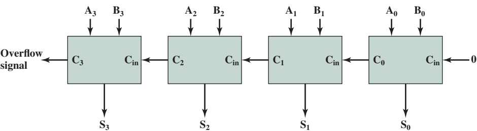
Figure 11.19 4-Bit Adder
