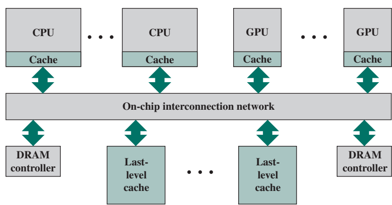
Figure 18.7 Heterogenous Multicore Chip Elements
