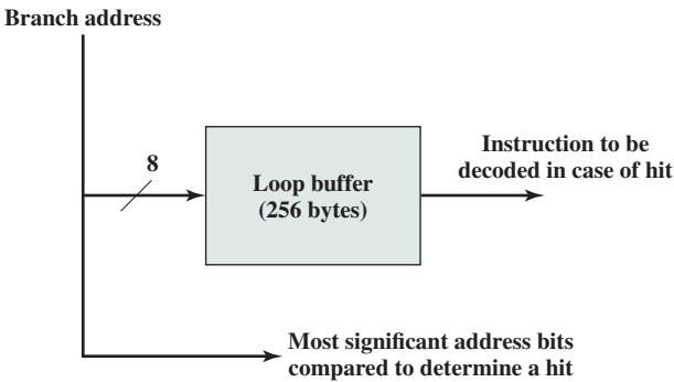
Figure 14.17 Loop Buffer
