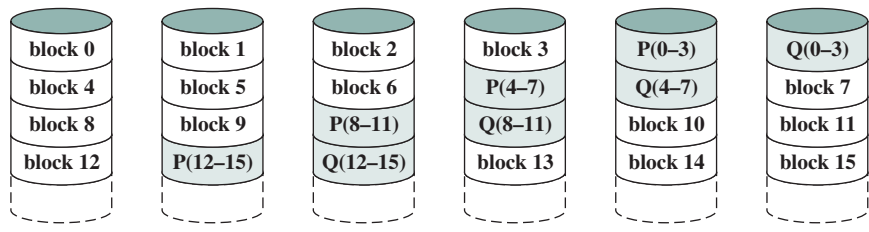
(g) RAID 6 (Dual redundancy)
