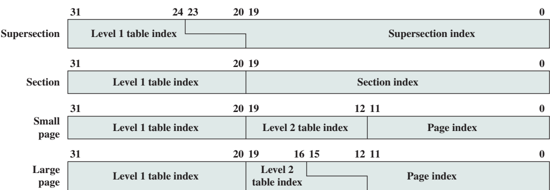
(c) Virtual memory address formats
