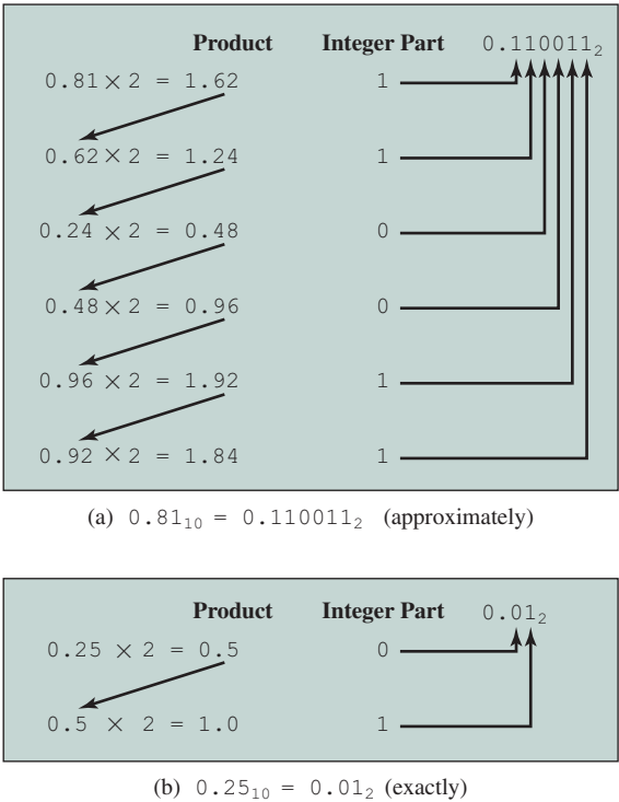
Figure 9.2 Examples of Converting from Decimal Notation to Binary Notation for Fractions
