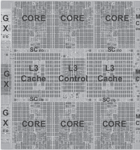
Figure 1.4 zEnterprise EC12 Processor Unit (PU) chip diagram Source: IBM zEnterprise EC12 Technical Guide, December 2013, SG24-8049-01. IBM, Reprinted by Permission
