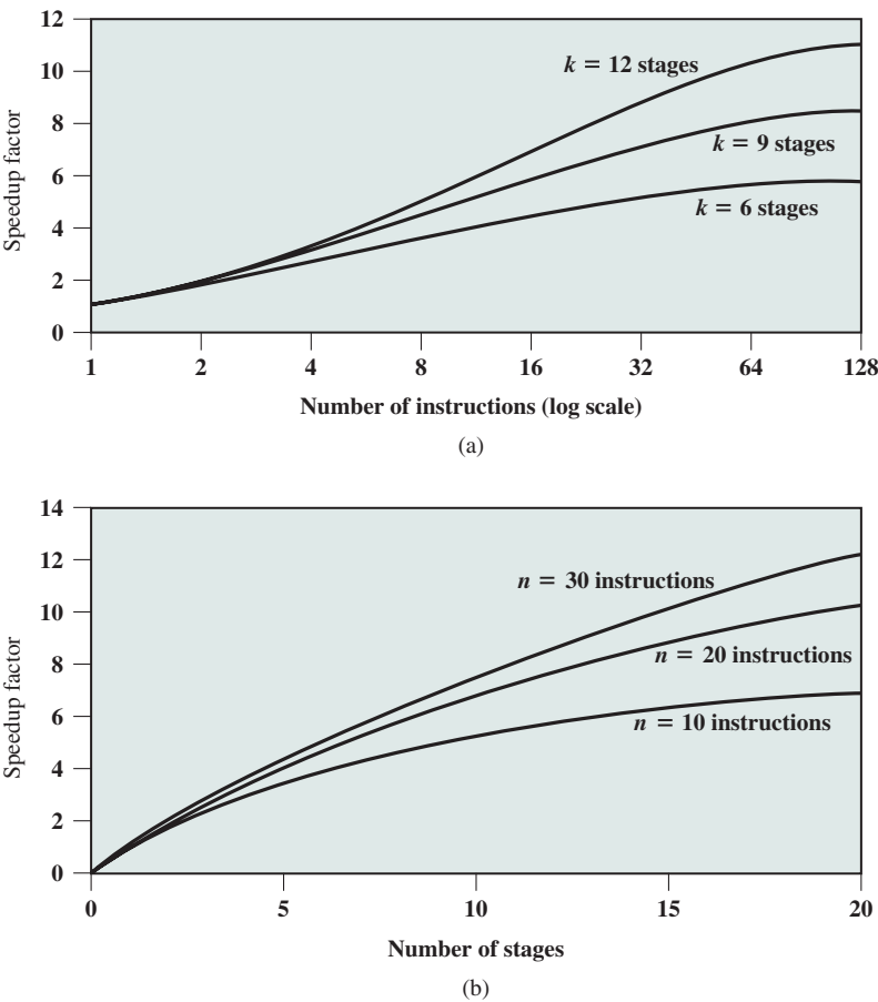
Figure 14.14 Speedup Factors with Instruction Pipelining
