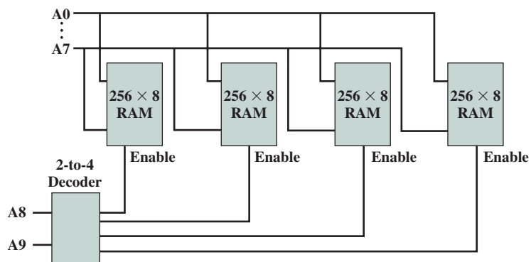
Figure 11.16 Address Decoding
