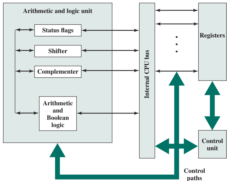
Figure 14.2 Internal Structure of the CPU
