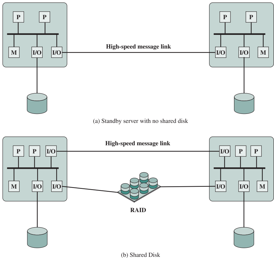
Figure 17.8 Cluster Configurations
